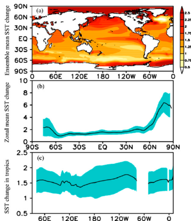
FIG. 1. (a) Ensemble mean of SST change patterns (K) in 17 CMIP5 models. Shown is global warming minus present day value. (b) Black line is the zonal mean SST changes, and shading stands for the uncertainty among different models. (c) Black line is the SST changes averaged between 5°S and 5°N, and shading shows the uncertainty of the zonal SST changes among the 17 models (one std deviation).
